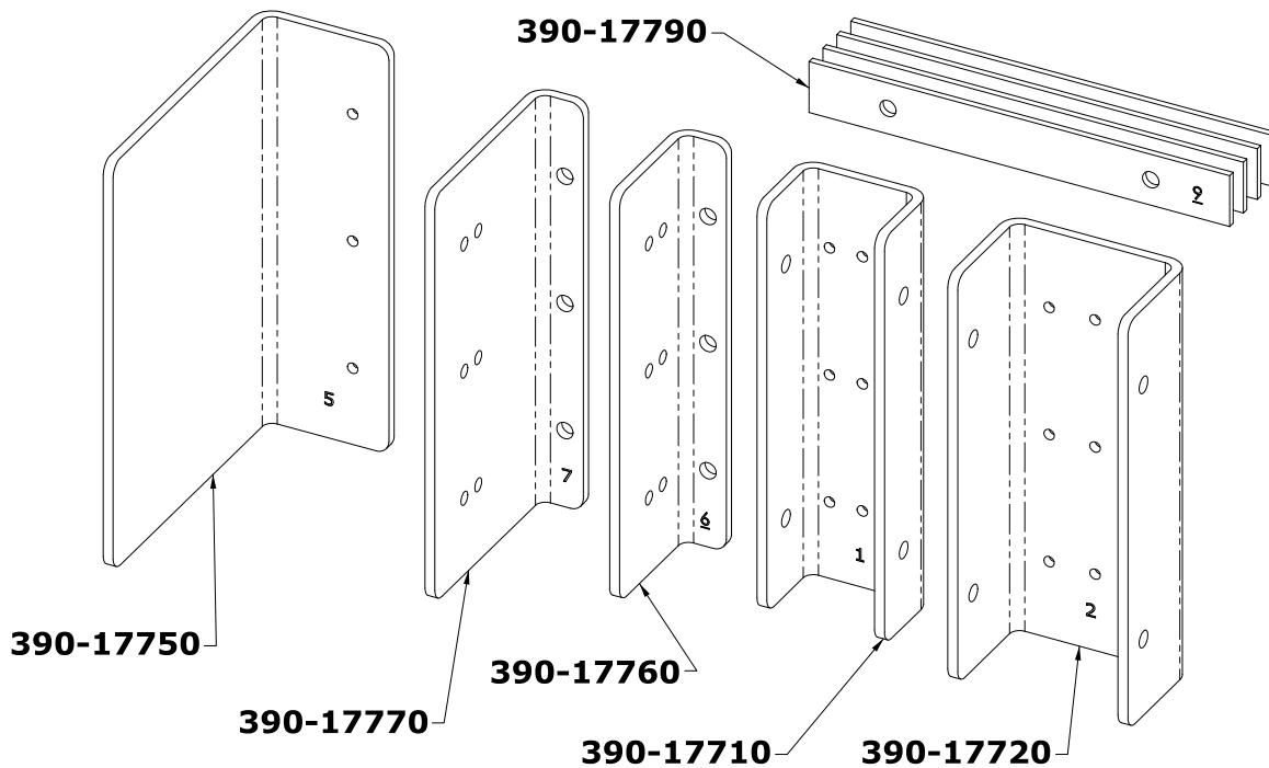
FMK-SW - Swing Gate Kit
