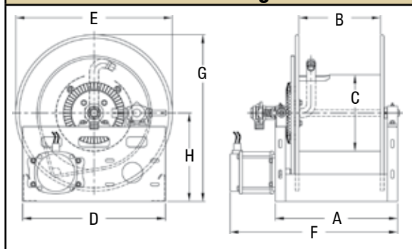
Dimensions Diagram
