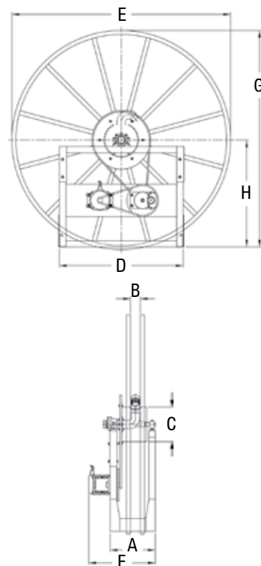
Dimensions Diagram
