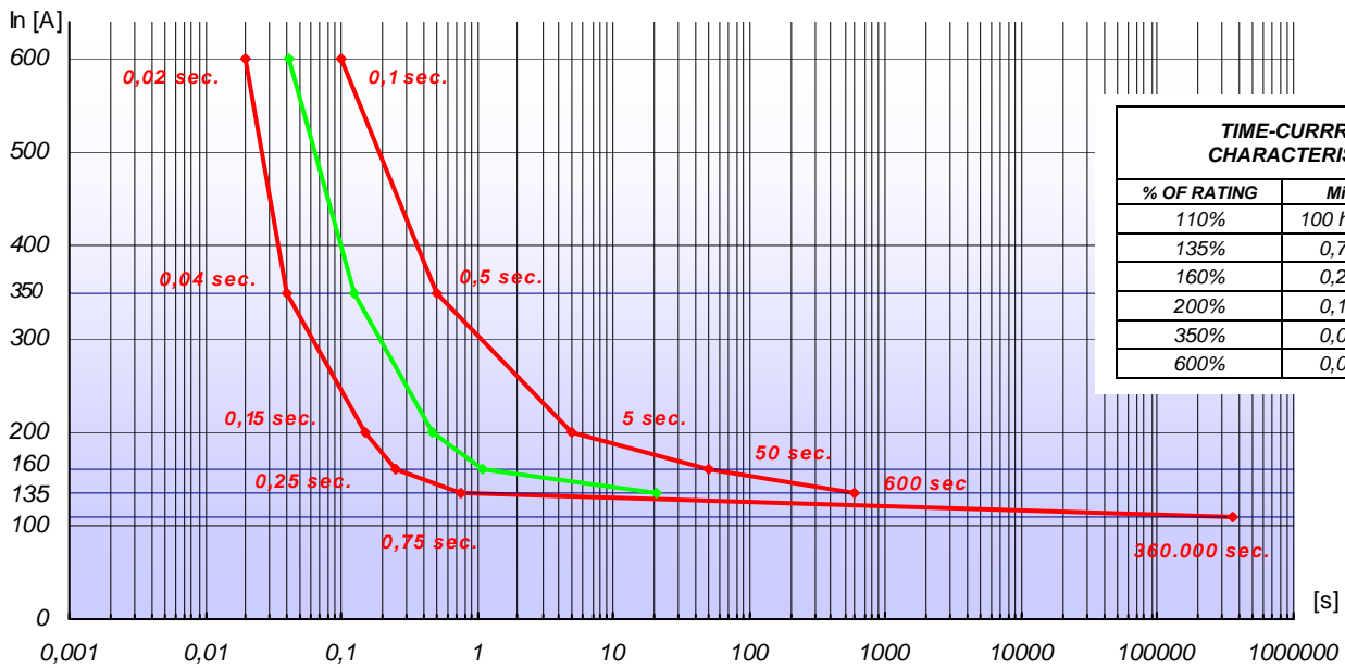
Example Fuse time-current curve (FORM C 10A) :
