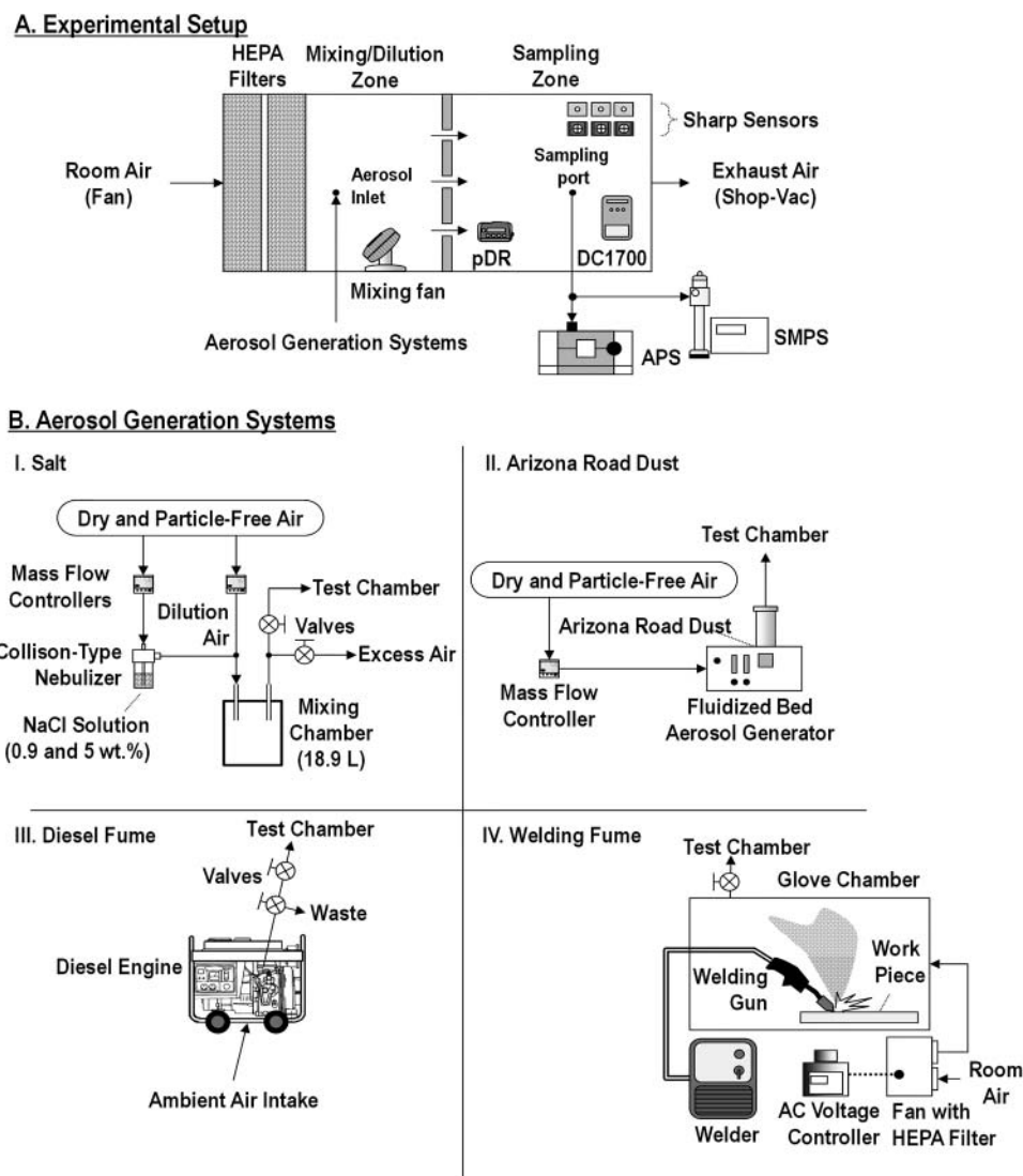
Figure 2. Experimental setup used to determine the performance of low-cost sensors shown in panel (a). Schematic diagrams of aerosol generation systems shown in panel (b).
