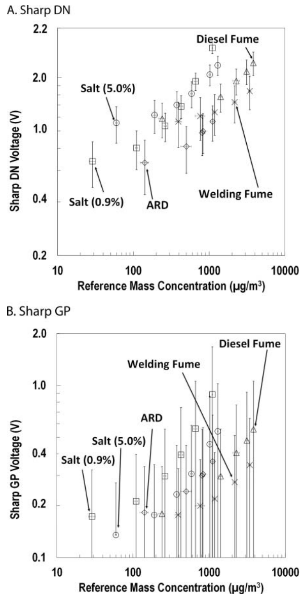
Figure 5. Raw output of the low-cost sensors relative to reference mass concentration for: (a) Sharp DN; (b) Sharp GP. Reference mass concentration was calculated by correcting SMPS + APS data with mass concentration measured with a gravimetric filter for each aerosol. The error bars represent one standard deviation.
