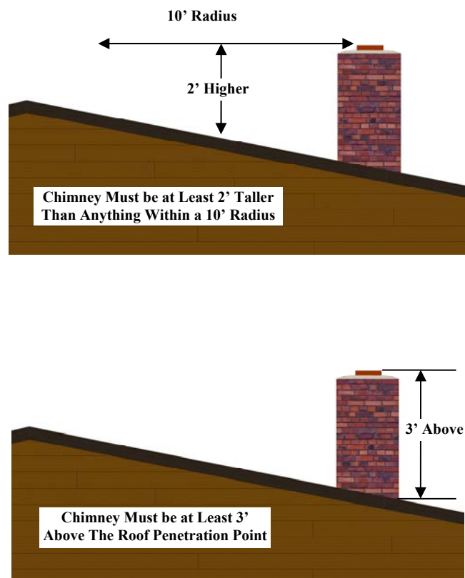
Figure 25. Chimney Height
